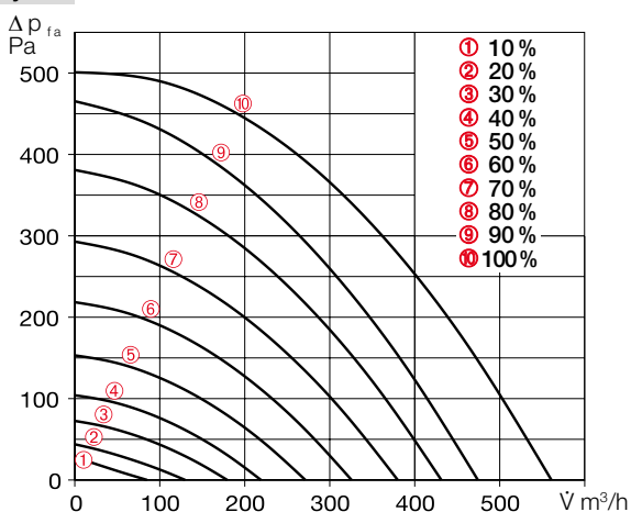
Characteristic curve KWL 500 W ET
