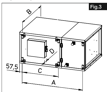
Suspension points
