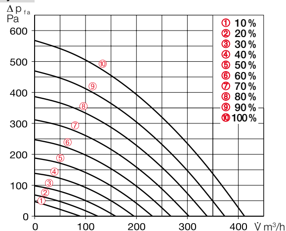
Characteristic curve KWL 360 W ET
