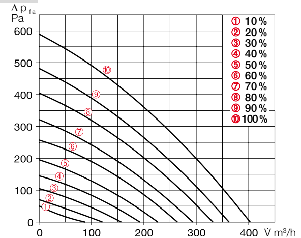
Characteristic curve KWL 360 W ET
