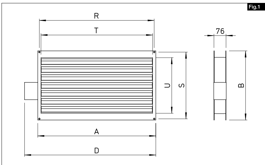
Dimensions Multi-leaf damper for AIR1 XC / XVP units
