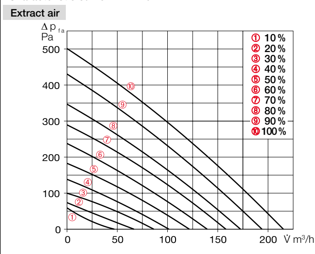
Characteristic curve KWL 170 W ET
