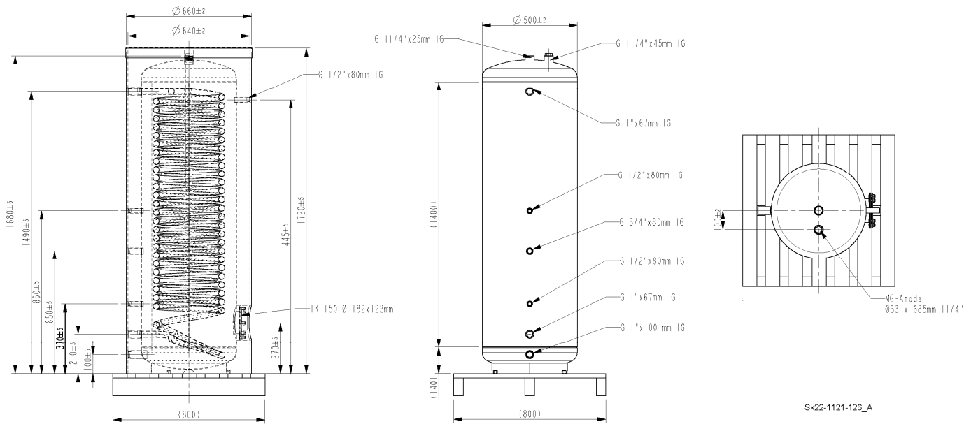
Abb. 20: THERAMAT WPS-300-1-F
