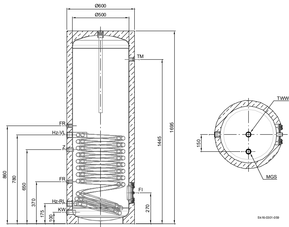
Abb. 8: THERAMAT EMH-300-1-F
