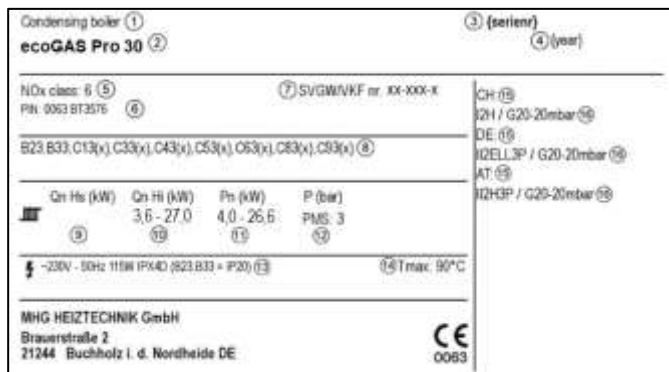
Abb. 99: Muster Typenschild ecoGAS Pro ... (Heizer)
