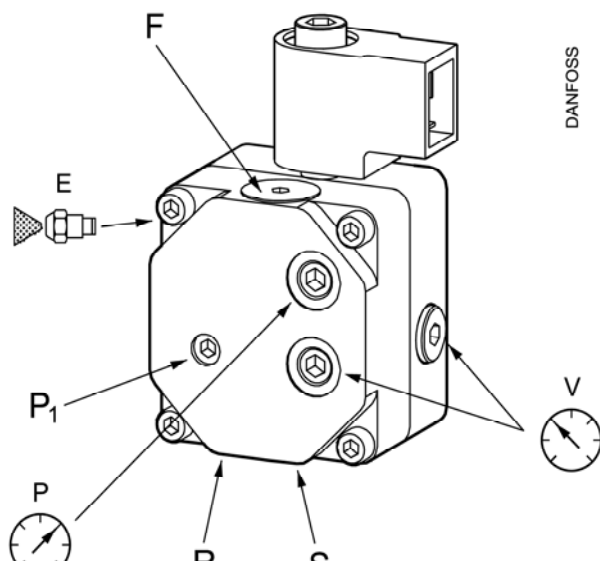
Abb. 16: Anschlüsse BFP 21 L4
