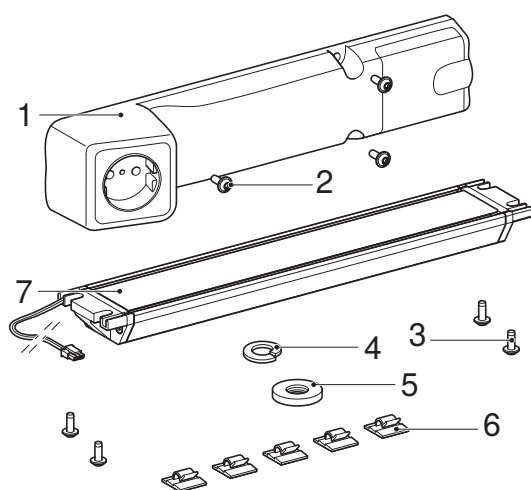
Figure 1: Geberit power socket element with ComfortLight module
