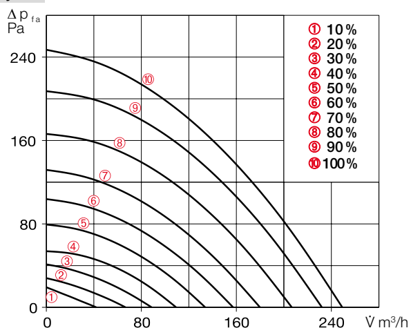
Characteristic curve KWL 300 W
