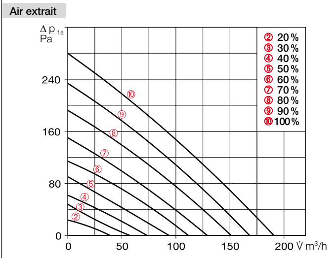
Characteristic curve KWL 200 W ET
