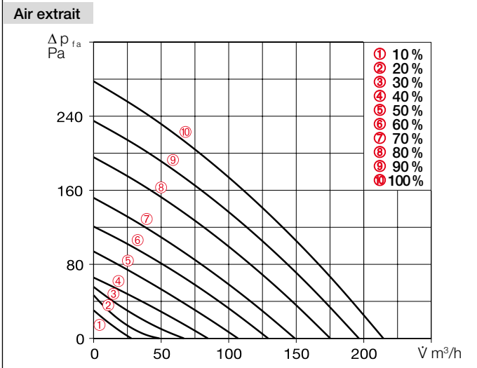
Characteristic curve KWL 200 W ET
