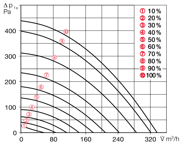
Characteristic curve KWL 300 W ET
