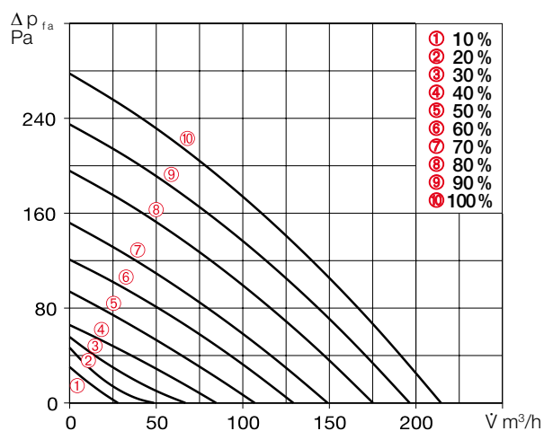
Characteristic curve KWL 200 W ET
