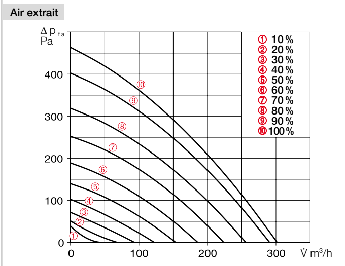
Characteristic curve KWL 300 W
