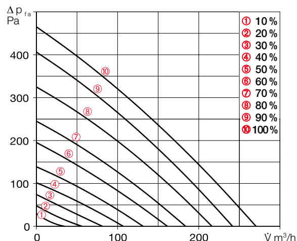
Characteristic curve KWL 300 W ET
