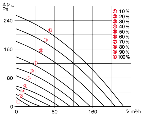
Characteristic curve KWL 200 W ET
